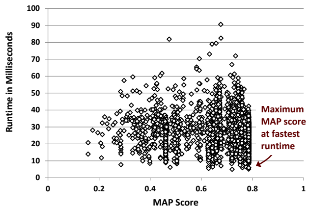
Figure 3: Runtime versus MAP output by the Genetic Algorithm during a search for the best software Artifact Connectivity configurations.
