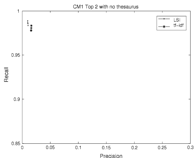
Fig. 7 Recall and precision for CM1 dataset, Top 2 feedback, no filter, LSI versus tf-idf
